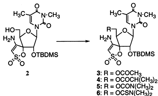
Scheme 1. Synthesis of spironucleosides ( 3–6 ).
