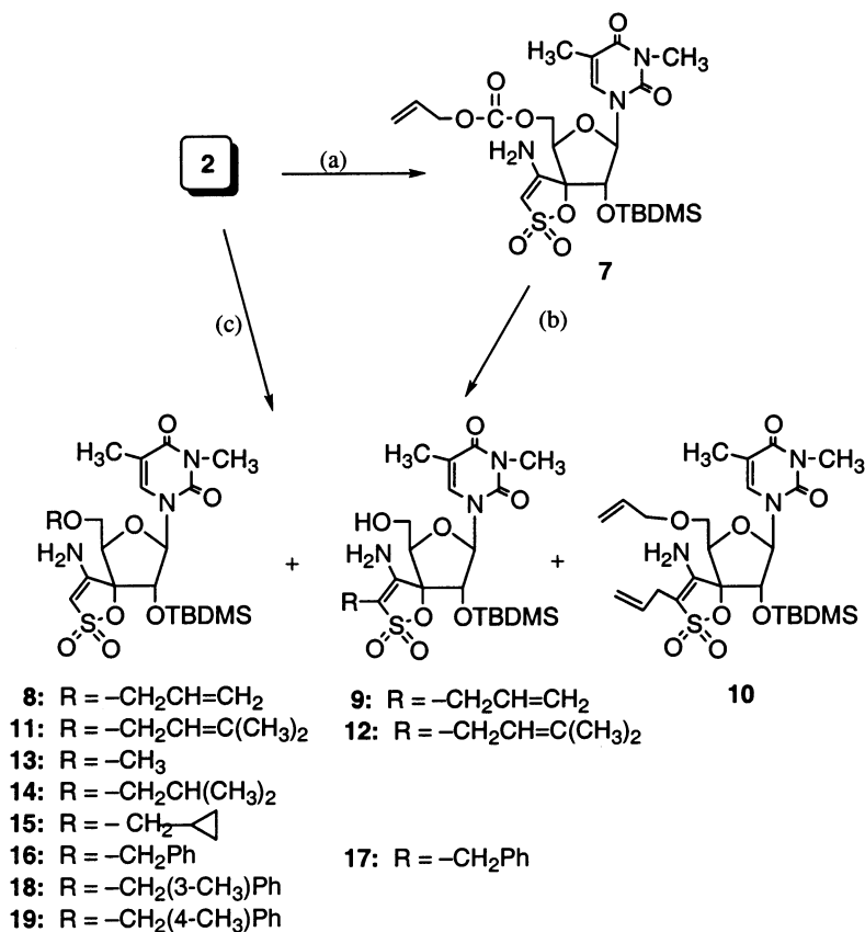
Scheme 2. Reaction conditions: (a) \text{ClCO}_2\text{CH}_2\text{CH}=\text{CH}_2 , THF, Pyridine; (b) \text{Pd}(\text{PPh}_3)_4 , THF; (c) NaH, RBr, DMF.
